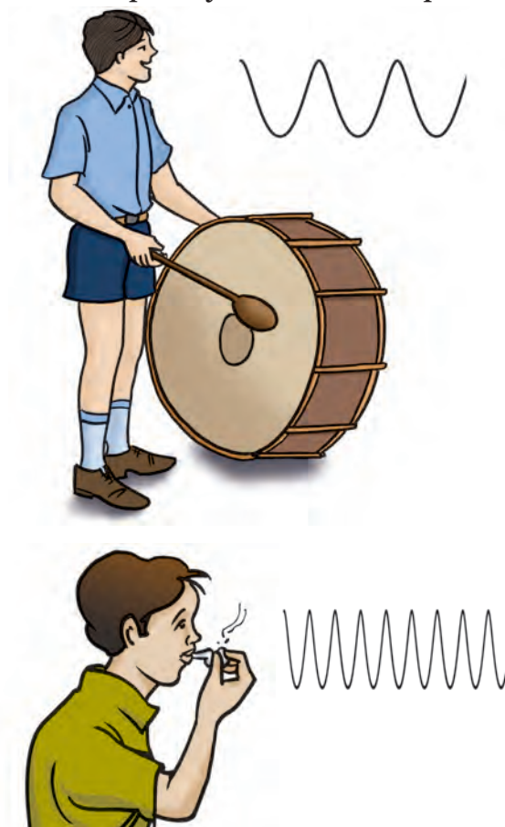
Fig. 10.18 : Frequency determines the pitch of a sound
